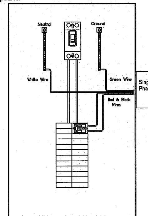
Location of Suppressor Shown with SPD breaker
